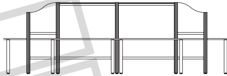
Fitz 6-way cluster. 1500h centre spine. 1350h end posts with curved polycarbonate panels
