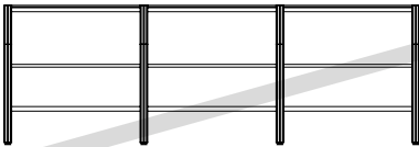
Carrel cluster. 1500h centre spine. 1200h privacy panels
