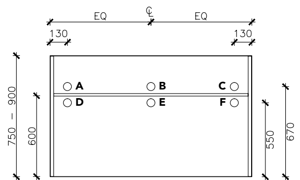
Rectangular Desk (750 - 900 Deep) Without Modesty - Location A, B, C With Modesty - Location D, E, F
