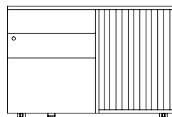
MMC1 900W x 500D x 610H
