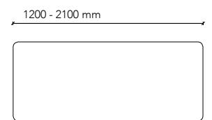
50 or 100 mm radius to all corners
