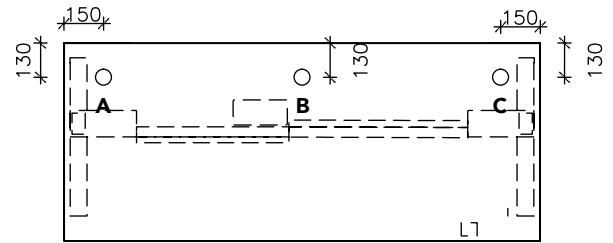
Rectangular Desk Standard Cable Port Location
