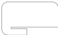
STRAIGHT Fits desk thickness 25 / 33mm only
