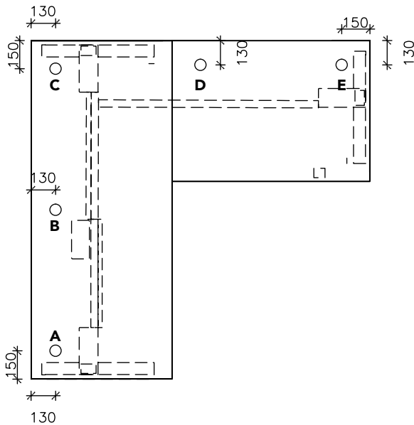
90° Corner Desk Standard Cable Port Location
