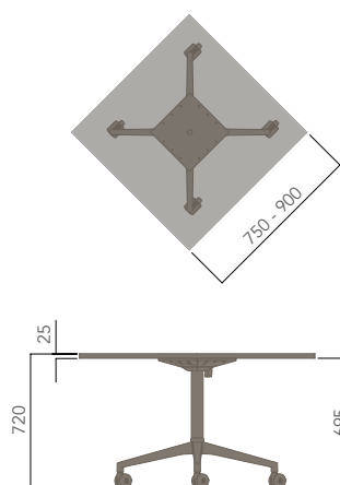
Square Top - 4 Star Folding Base (Castors)
