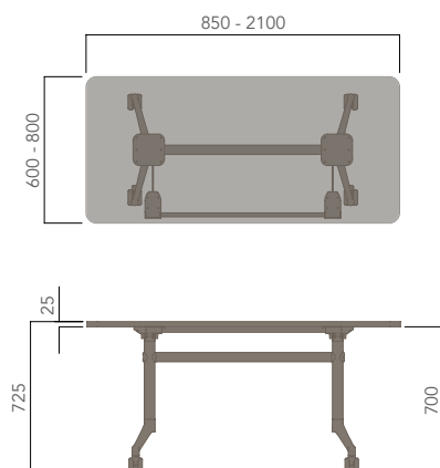
Rectangular Top - Folding Base (Castors)
