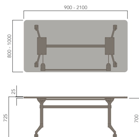
Rectangular Top - Folding Base (Castors)
